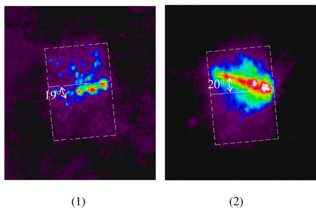
FIG. 8. (Color online) Microscope images for beam steering by wavelength: (1) beam angle at 1546 nm and (2) beam angle at 1572 nm.
