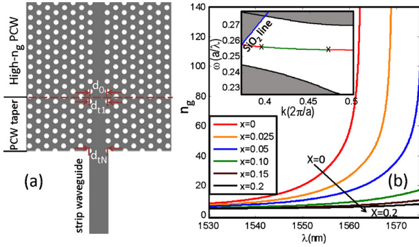
FIG. 1. (Color online) (a) A schematic of the strip waveguide to high- n_g photonic crystal waveguide coupling structure. The PCW on the right side of the interface is assumed to support high- n_g propagation at the wavelength of operation. (b) Group index vs wavelength for infinitely long PCW with different defect line widths, d_0=a(\sqrt{3}+x) . The inset shows band structure for W1 PCW, r=0.26a , slab thickness=230 nm, n(\text{SiO}_2)=1.45 , and n(\text{Si})=3.47 . The highlighted (green) section is the bandwidth over which 20 < n_g < 100 .
