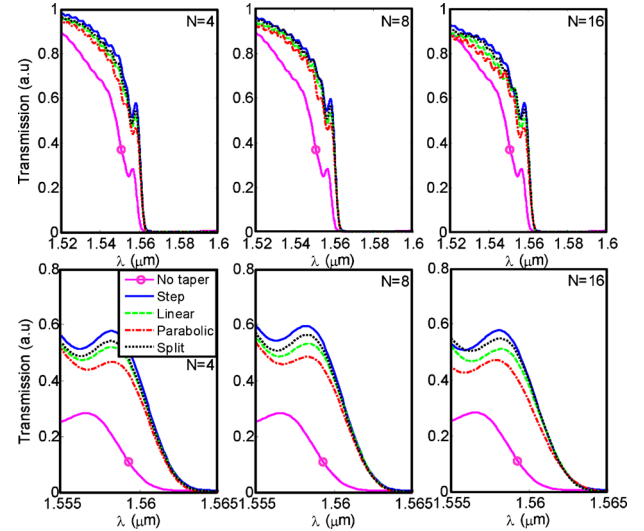
FIG. 2. (Color online) 3D FDTD simulation results for direct coupling of strip waveguide and PC slab waveguide (no taper) and coupling through PCW tapers, with step, linear, parabolic, and split profiles, for N=4, 8 , and 16. The lower row graphs were zoomed at the band-edge region.
